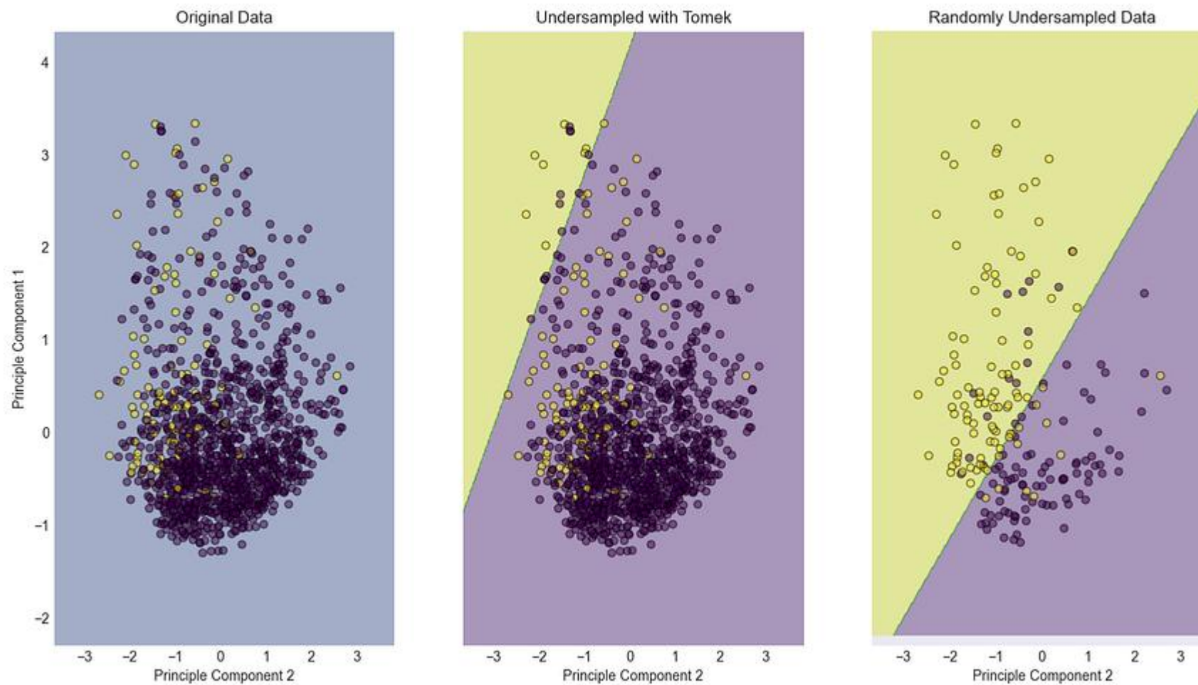
Comparing the Different Undersampling Methods
