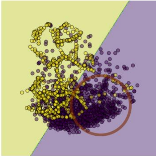
Oversampling with SMOTE
